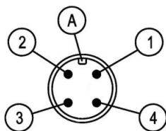
Fig. 3: M12 connector 4-pin
