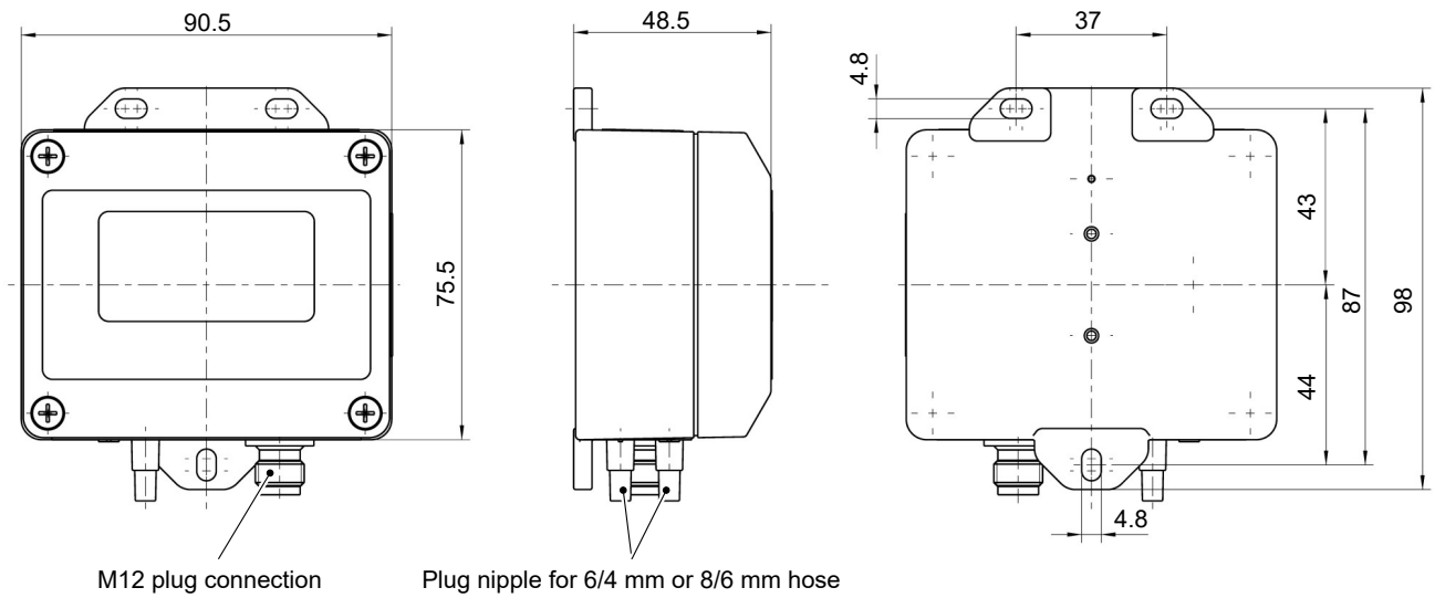
Fig. 4: Dimensional drawing
