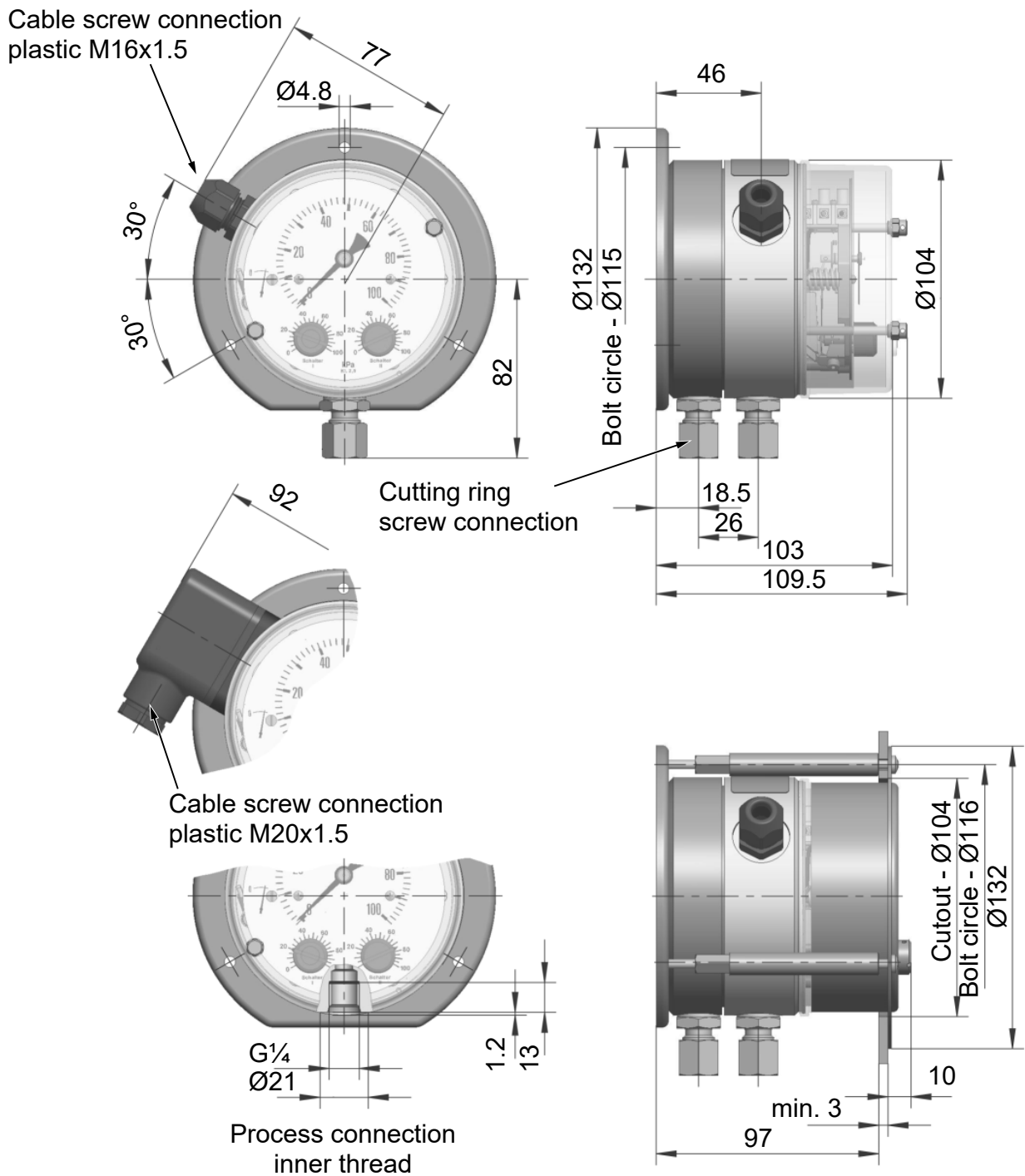
Fig. 8: Pressure chamber in VA (IP55)
