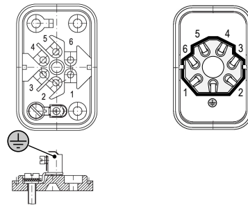
Fig. 5: Cable socket / plug
