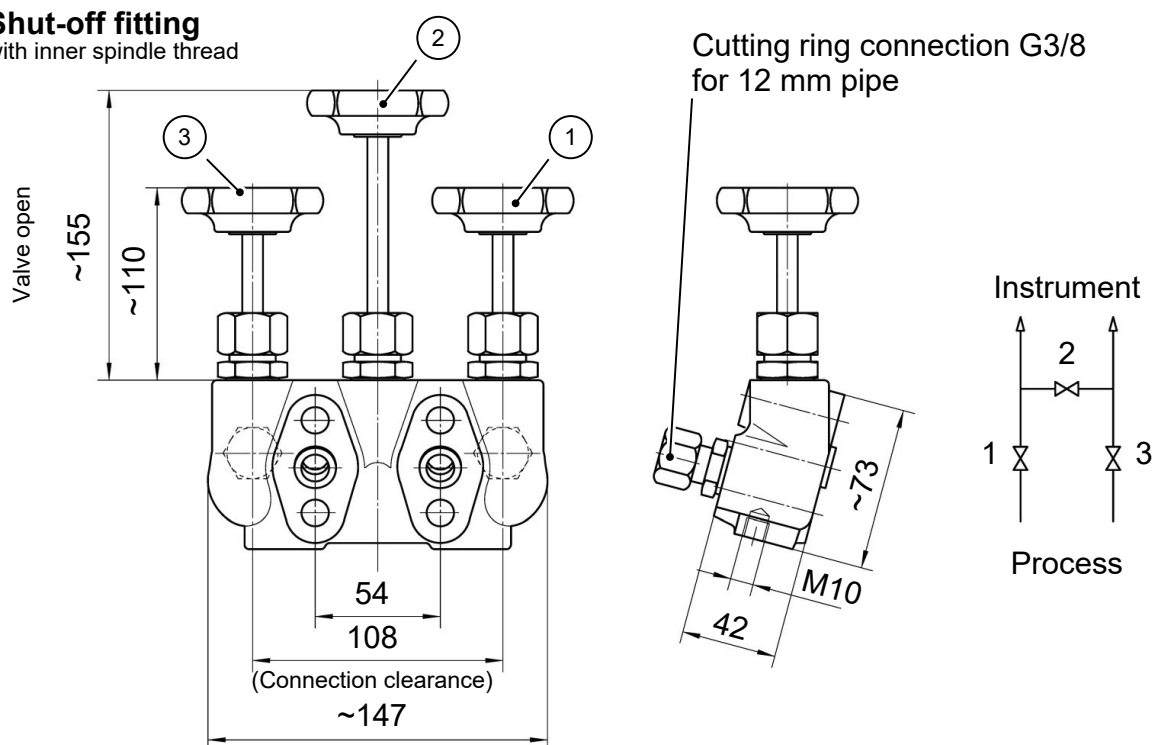
Fig. 28: Shutoff valve DZ3600SV2700
