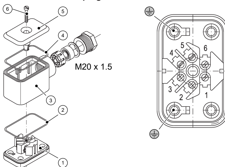
Fig. 12: Cable socket
