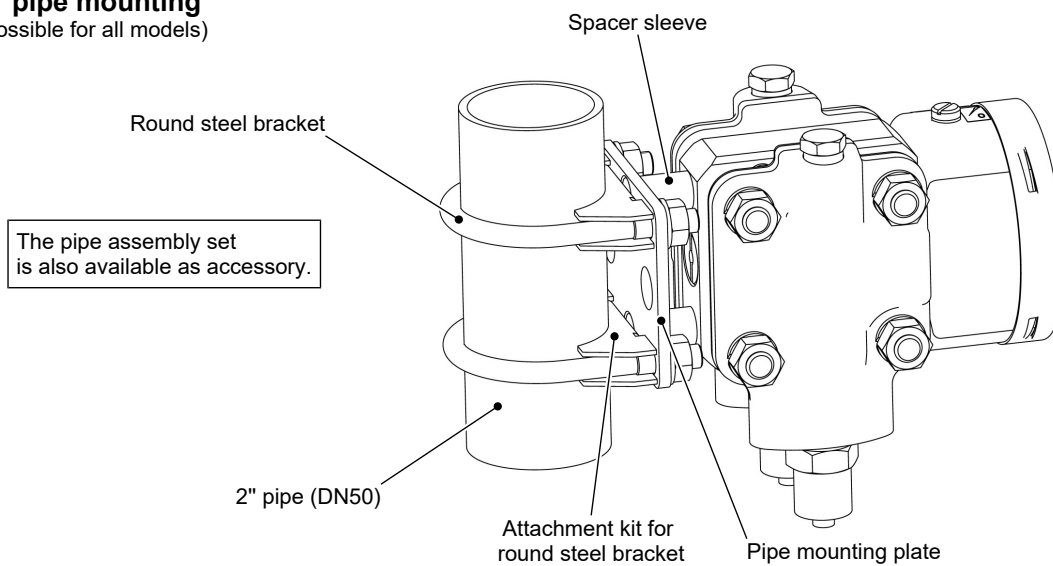
Fig. 23: Pipe mounting
