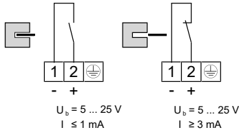
Fig. 15: Inductive contact
