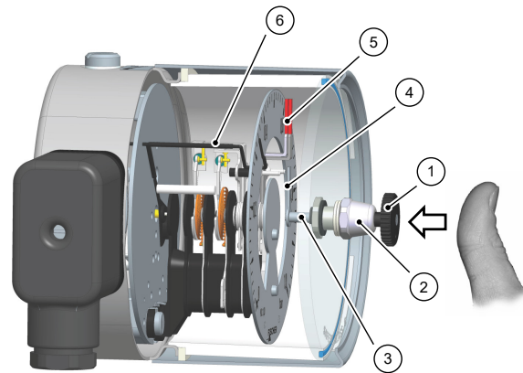
Fig. 20: Switch point setting
