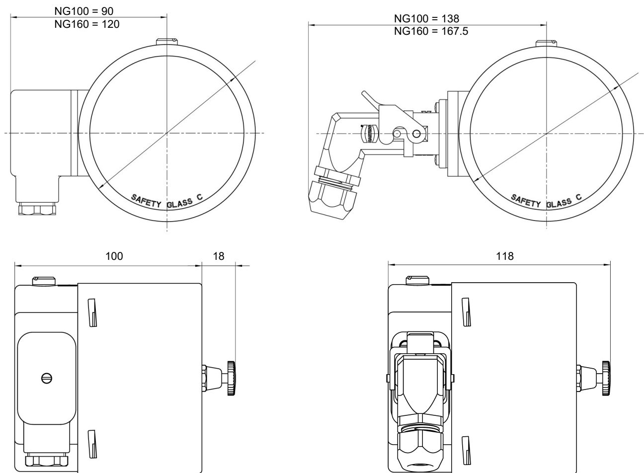
Fig. 27: Dimensional drawing contact devices
