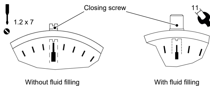
Fig. 19: Zero point correction screw
