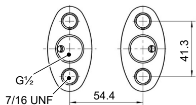
Fig. 22: Dimensional drawing (Small measuring system Ø75)
