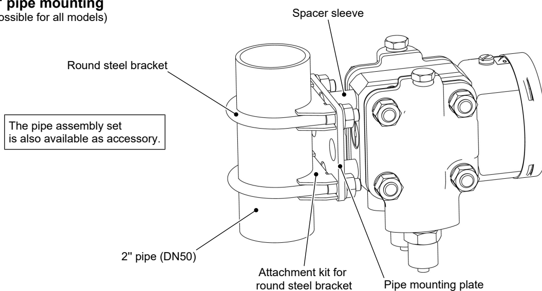
Fig. 20: Pipe mounting
