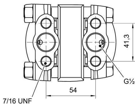
Fig. 19: Dimensional drawing (Small measuring system Ø75)
