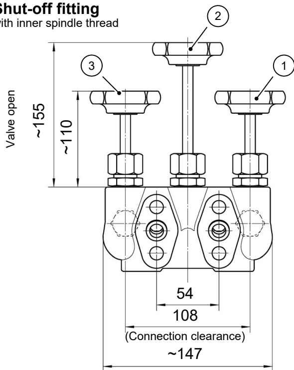
Fig. 24: Shutoff valve DZ3600SV2700
