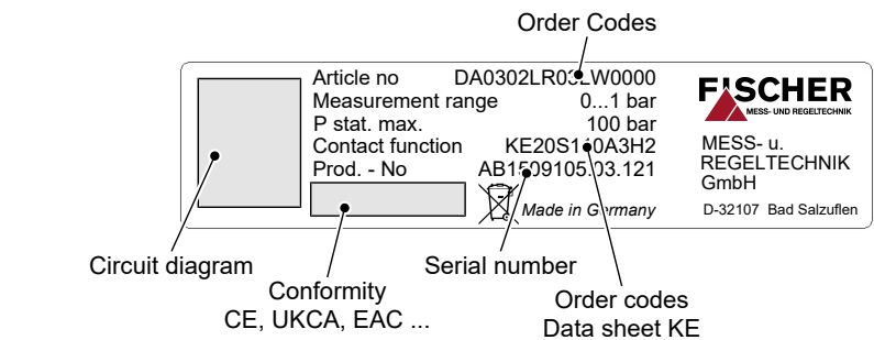
Fig. 3: Nameplate
