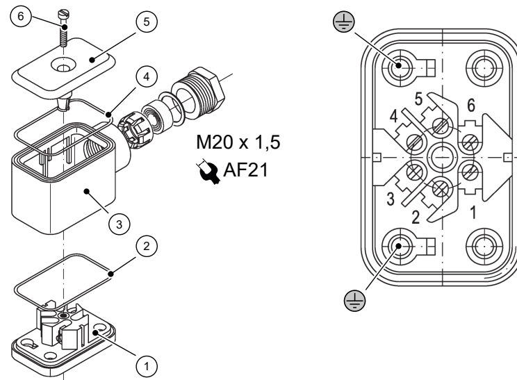
Fig. 9: Cable socket
