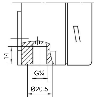
Fig. 8: Inner thread G \frac{1}{4}
