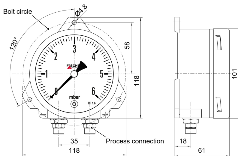
Fig. 7: Dimensional picture
