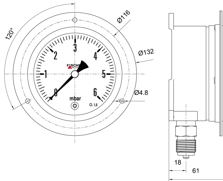
Fig. 12: Connections bottom
