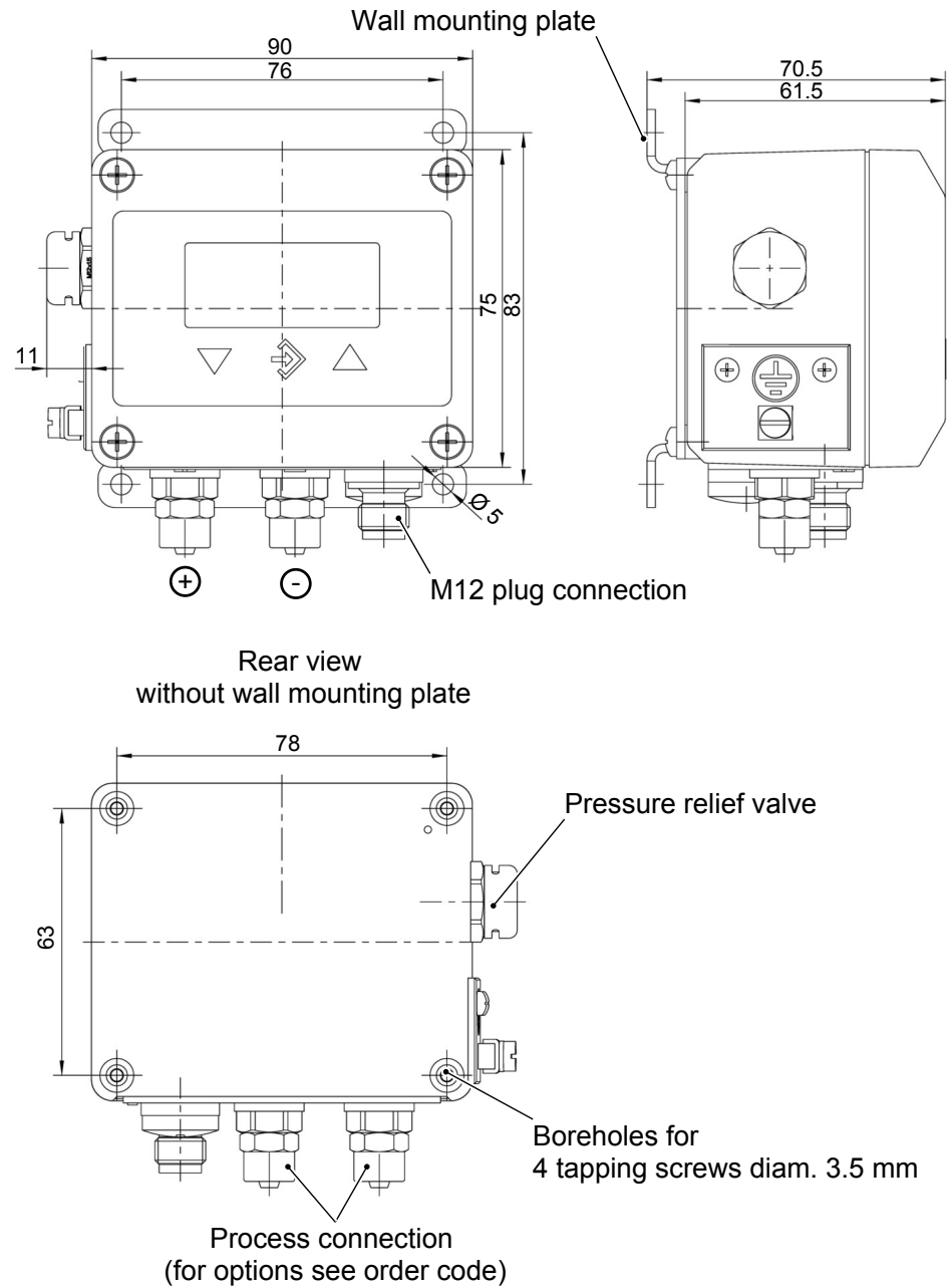
Fig. 11: Dimensional picture
