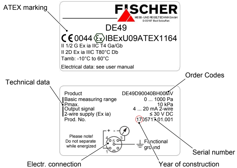
Fig. 2: Nameplate
