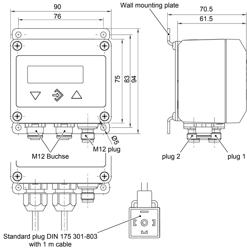
Fig. 19: Dimensional picture
