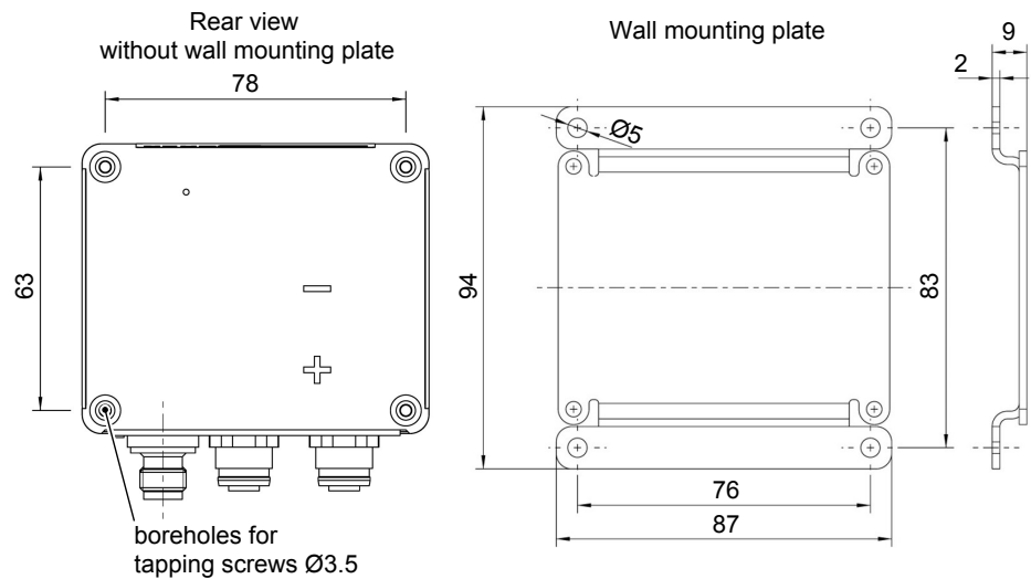
Fig. 20: Wall mounting
