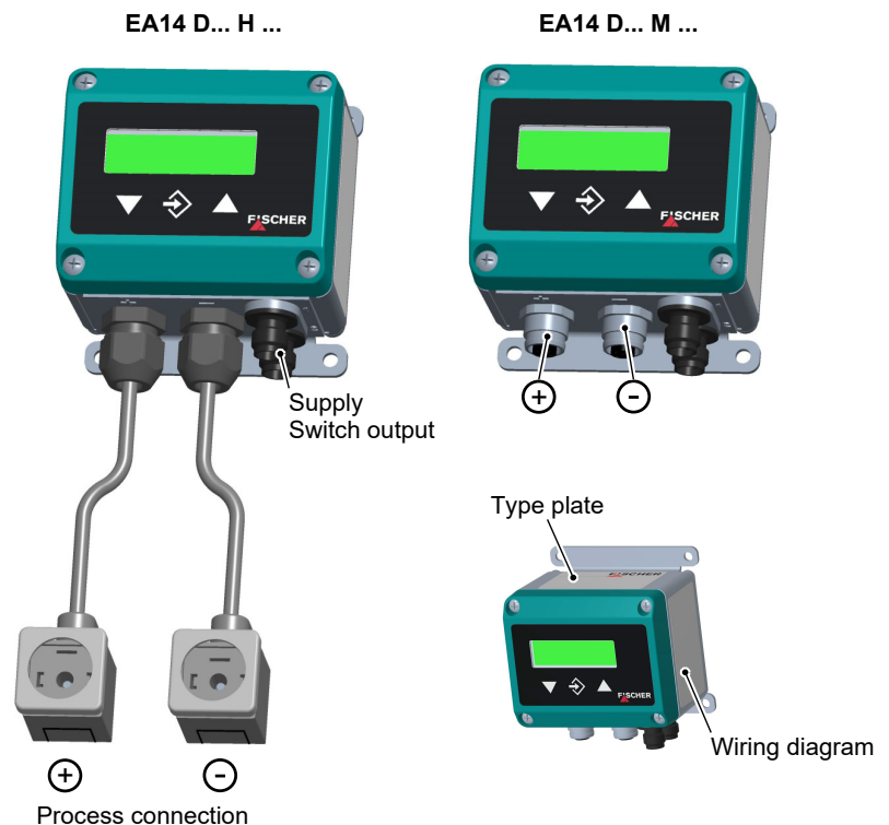
Fig. 2: Equipment versions
