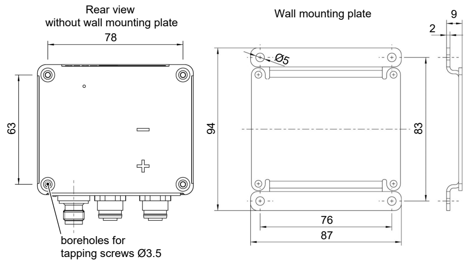
Fig. 20: Wall mounting
