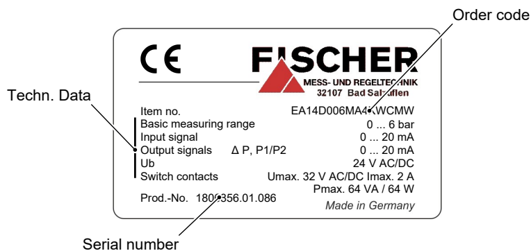
Fig. 4: Type plate
