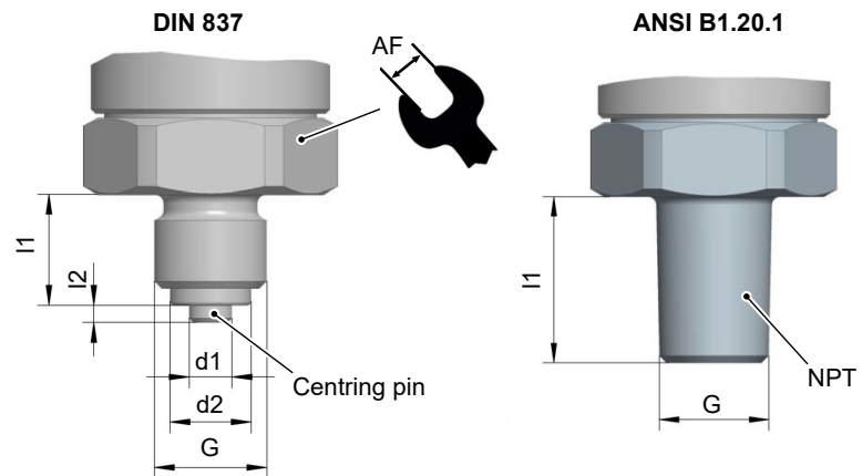
Fig. 16: Connecting shanks
