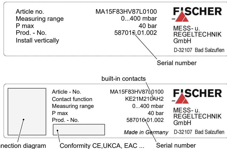
Fig. 3: Type plates with and without contacts
