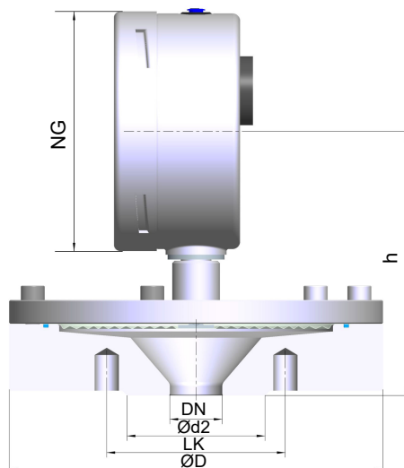
Fig. 15: Connection flange
