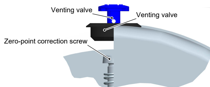
Fig. 9: Zero point correction
