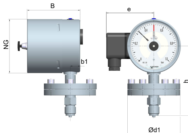
Fig. 13: Dimension drawing MA15F with contacts
