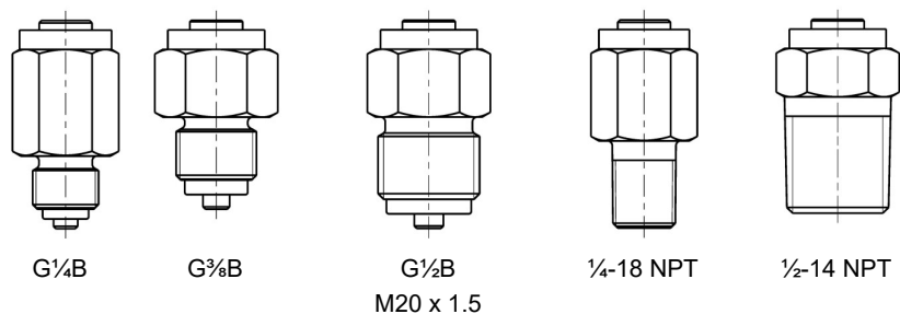
Fig. 2: Process connection
