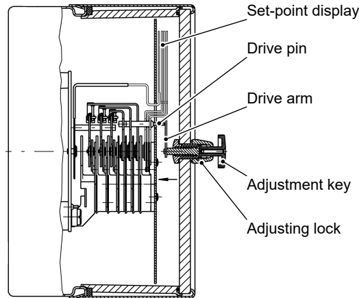
Fig. 11: Contact element
