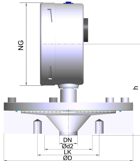
Fig. 15: Connection flange
