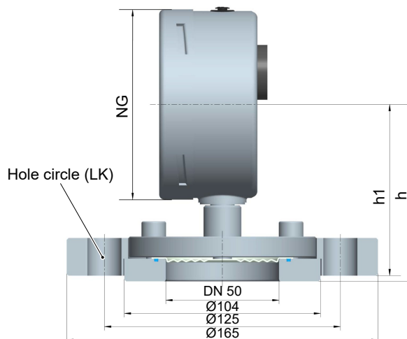
Fig. 14: Collar flange
