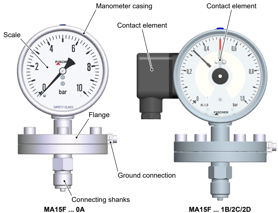
Fig. 1: Product summary
