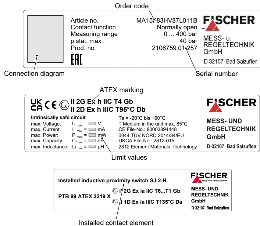
Fig. 3: Name plate
