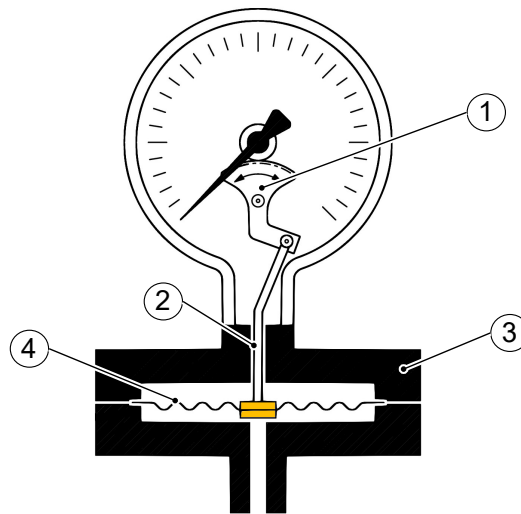
Fig. 4: Function diagram
