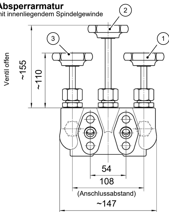
Abb. 18: Absperrventil DZ3600SV2700
