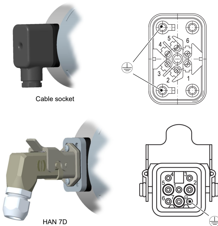
Fig. 10: Cable socket
