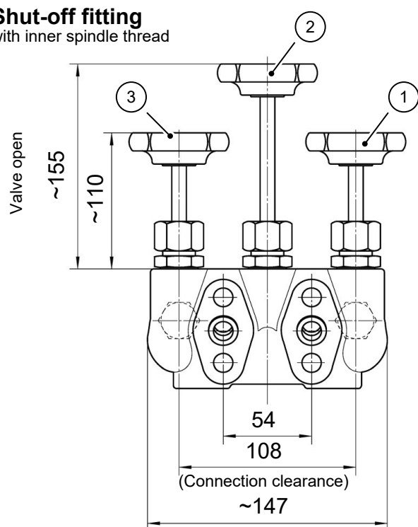
Fig. 17: Shutoff valve DZ3600SV2700
