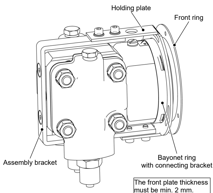
Fig. 14: Installation of front panel with panel fittings
