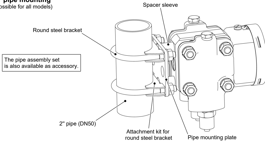
Fig. 12: Pipe mounting
