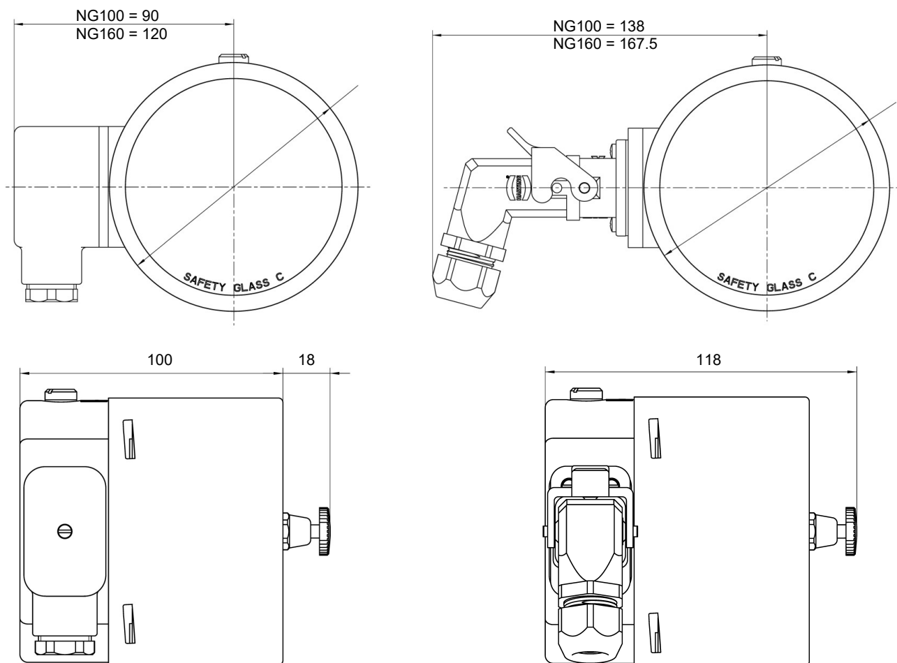
Fig. 16: Dimensional drawing contact devices
