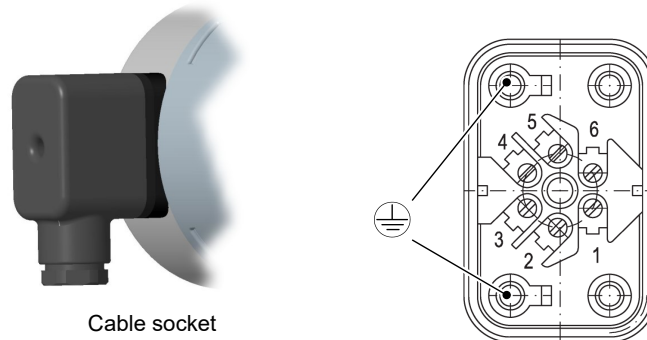
Fig. 11: Cable socket
