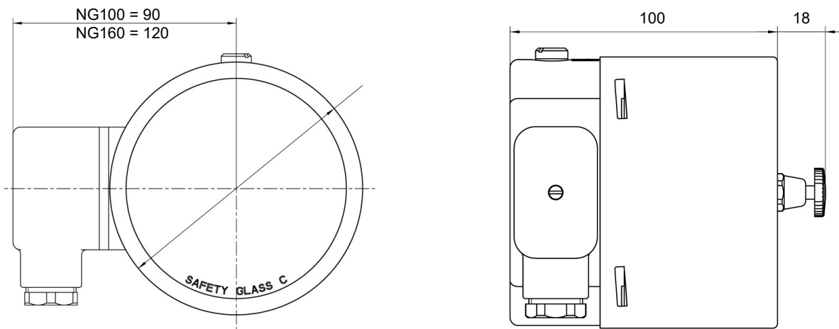
Fig. 17: Dimensional drawing of contact device
