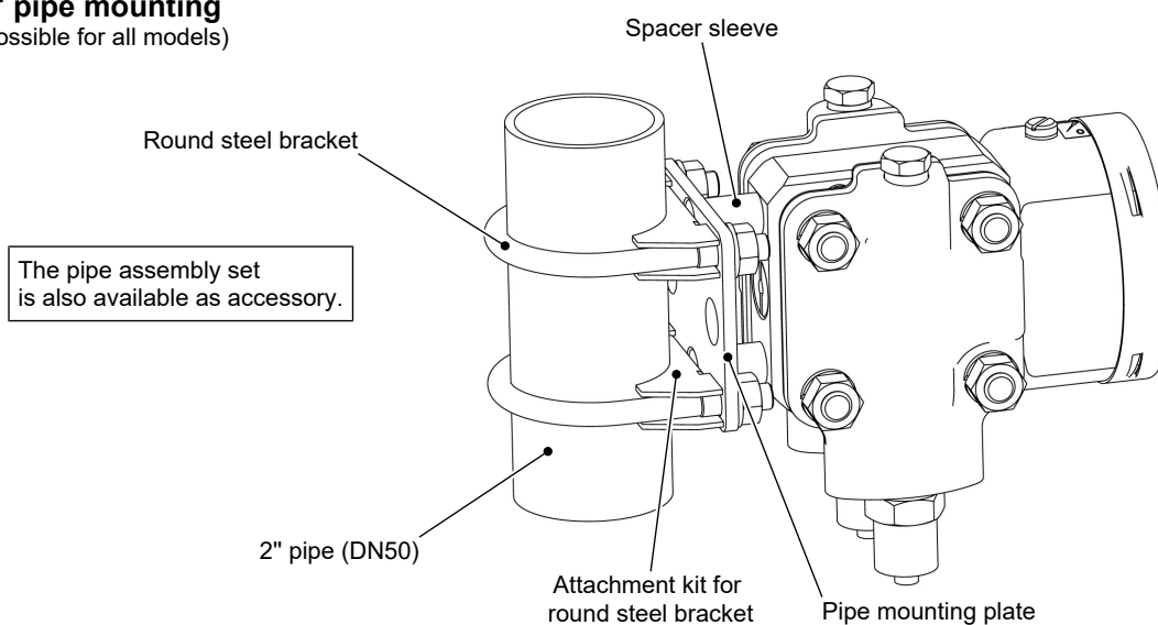
Fig. 9: Pipe mounting
