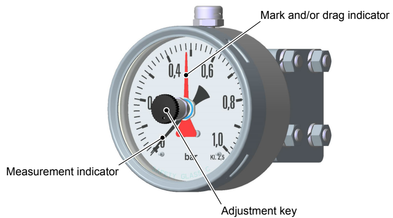
Fig. 2: Needle
