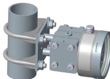
Tube assembly
