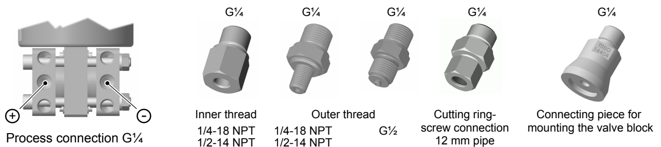
Fig. 4: Options for the process connection
