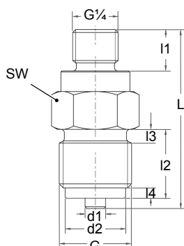
Fig. 11: Connecting port G
