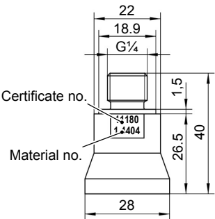
Fig. 15: Connecting piece
