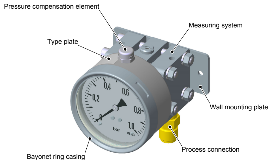
Fig. 1: Device overview
