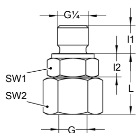
Fig. 14: Screw-in connection
