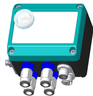
Pneumatic plug connection for 6/4 or 8/6 mm hose
