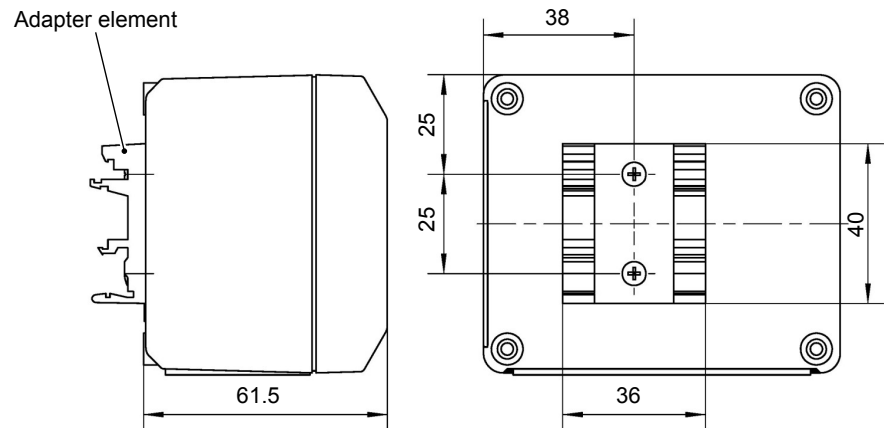
Fig. 6: Adapter element
