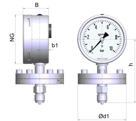
Fig. 3: Dimension drawing MA15F without contacts
