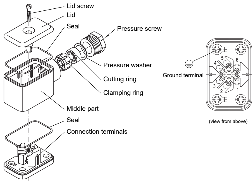
Fig. 5: Cable socket
