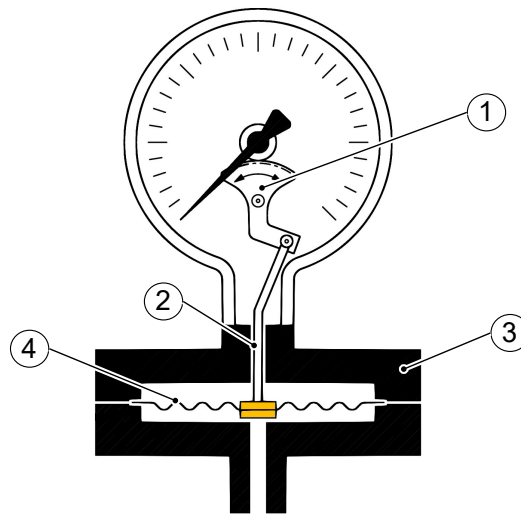
Fig. 2: Function diagram
