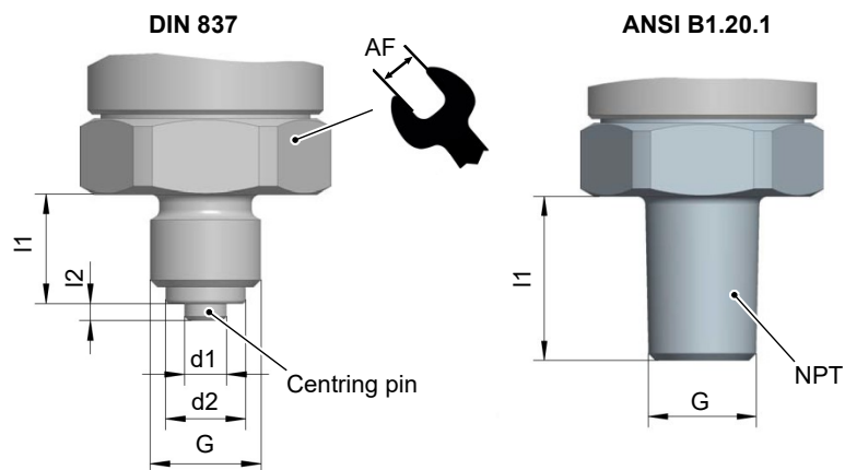
Fig. 8: Connecting shanks
