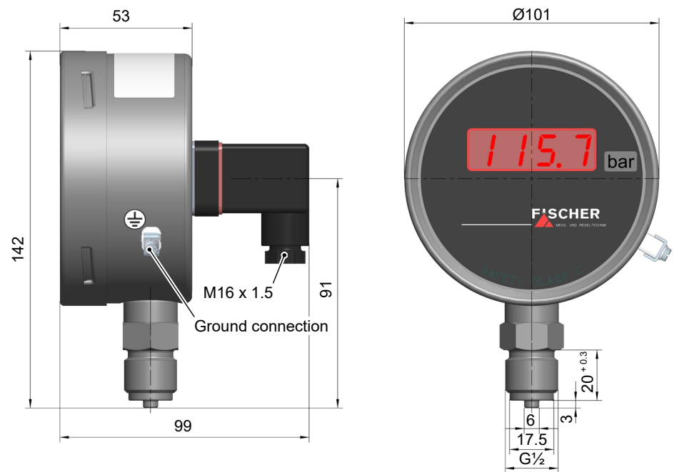
Fig. 3: Dimensional drawing
