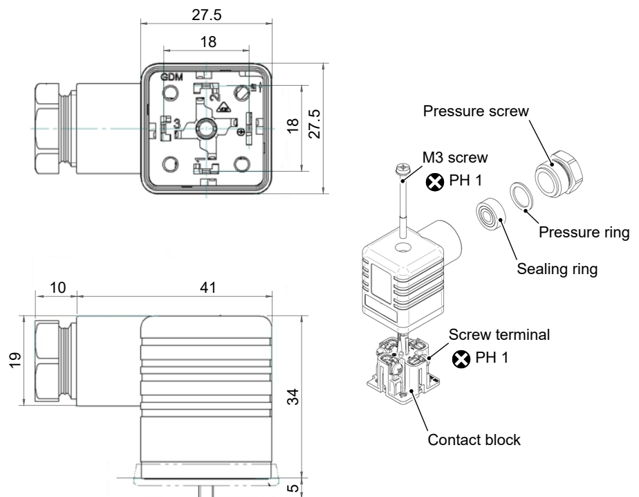
Fig. 3: Dimensional drawing
