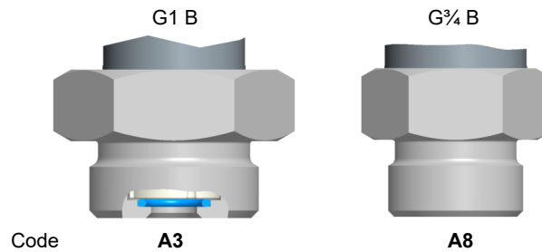
Code A3 A8 Fig. 2: Process connections
