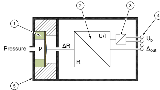
Fig. 3: Function diagram
